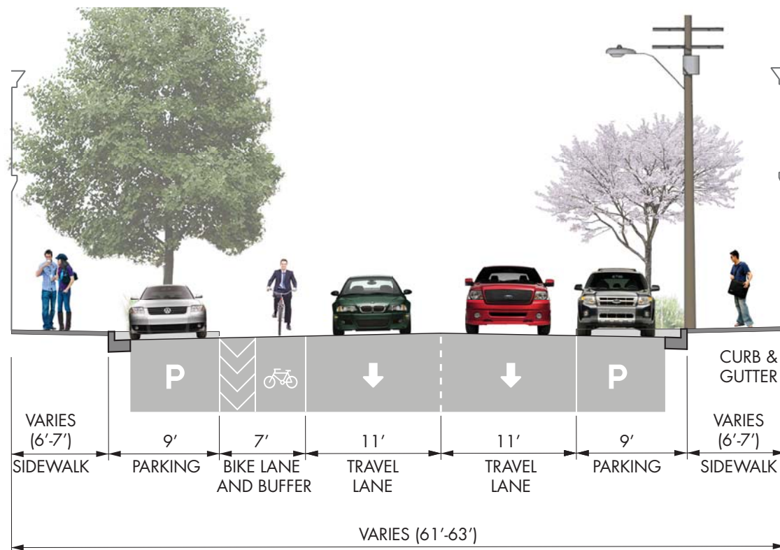
SECTION A-A [COLLEGE STREET LOOKING EAST]
