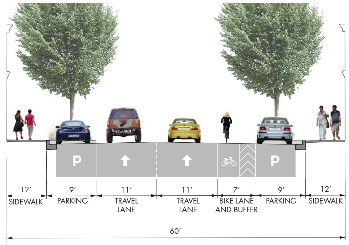
SECTION B-B [STATE STREET LOOKING EAST]
