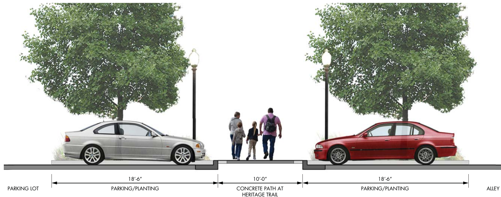
SECTION A-A [AT MUNICIPAL PARKING LOT]
