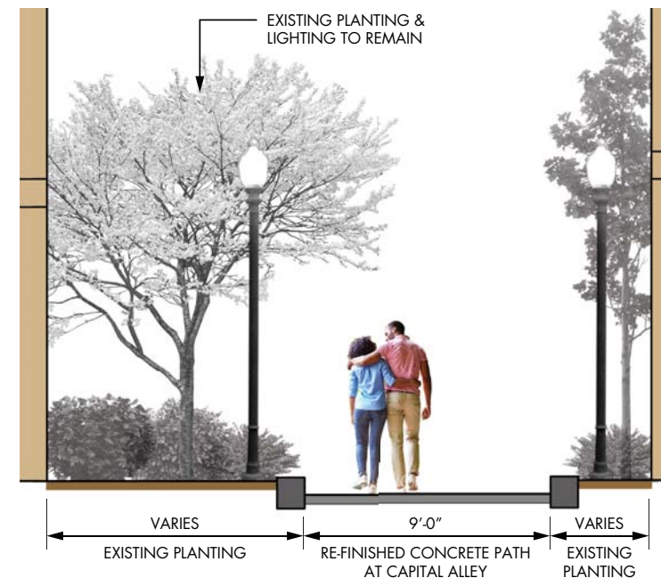
SECTION C-C [AT CAPITAL ALLEY]
